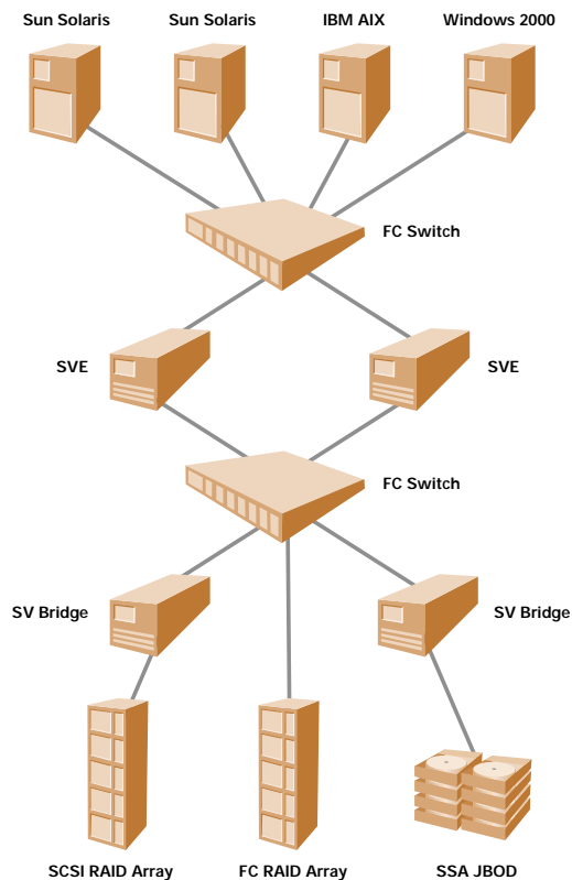
Sample of Vicom SVE in a heterogeneous SAN topology
